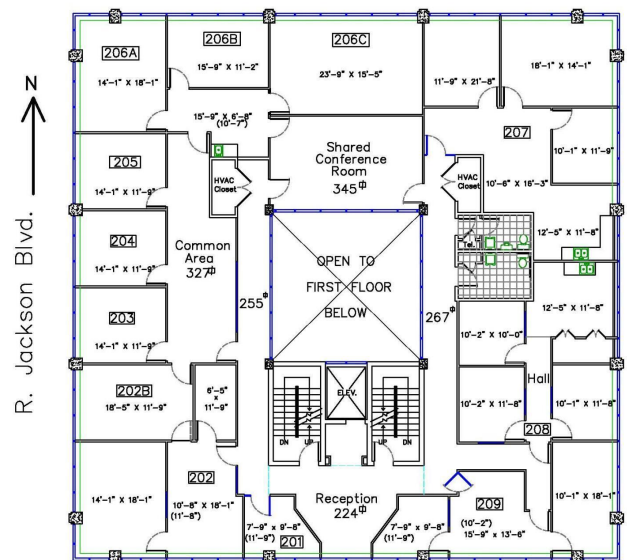
2nd Floor Level Plan
