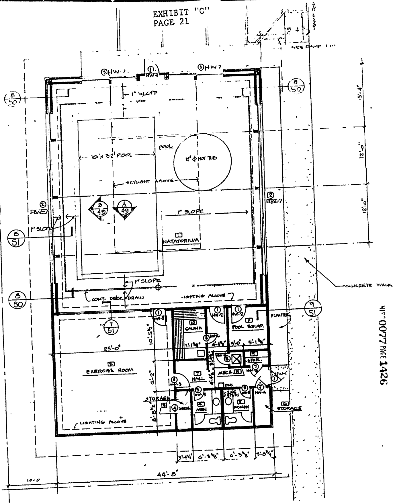
FLOOR PLAN - INDOOR POOL BLDG. SCALE: 1/8" = 1'-0"
