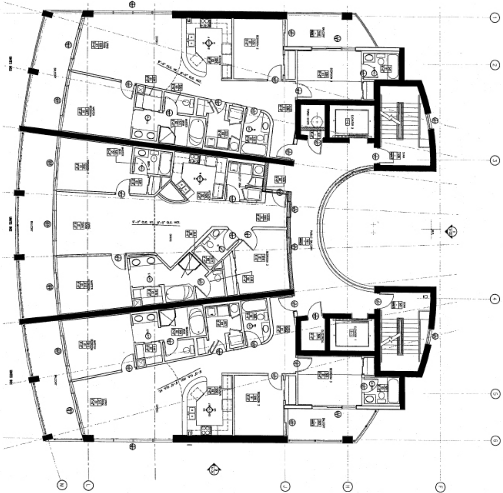
1 NINTH FLOOR PLAN 1 1/2" = 1'-0" 2001 - 11/17/07
