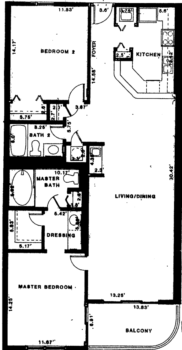
TYPE 2 2 BEDROOM 2 BATH SHEET #3
