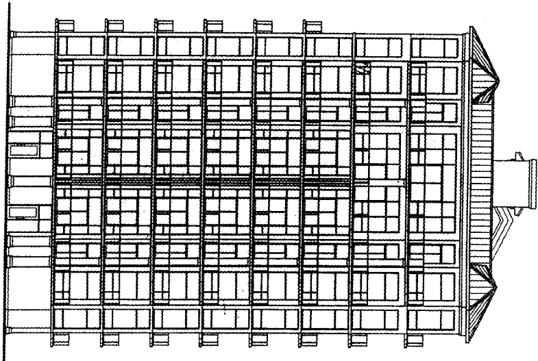
① SOUTH ELEVATION 0 5' 10' 20'
